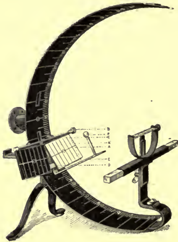
FIG. 225.—Tortometer of the author arranged for measuring torsion in various planes.
